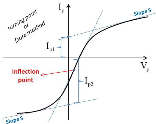
Figure 2. Schematic diagram of the double probe characteristic to determine T_e in turning point or Dote method [45].
