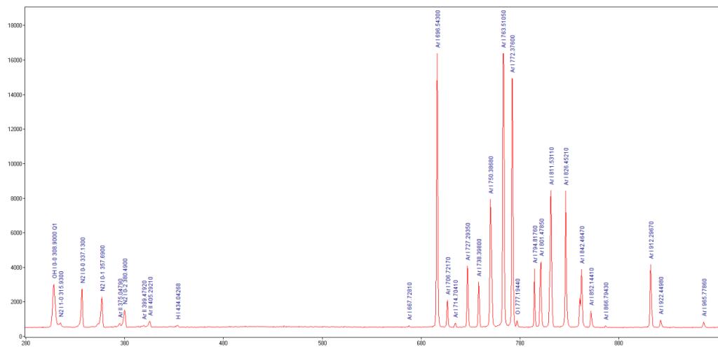
Figure 11. Optical emission spectrum at middle of the plasma plume (position 2) with an applied power of 30 W and gas flow rate of 4.5 slm.
