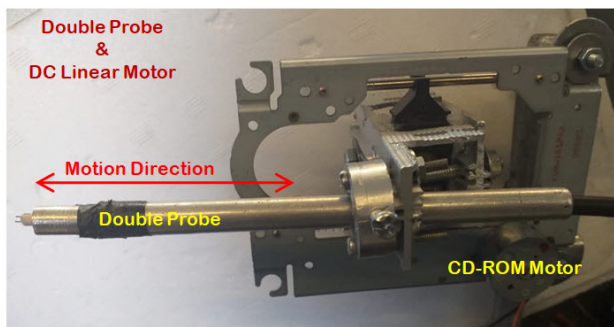
Figure 7. Langmuir double probe on the linear reciprocating system which has been constructed using a CD-ROM DC motor.
