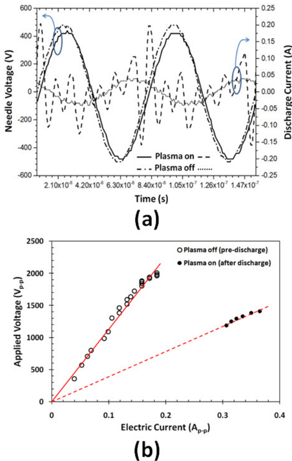
Figure 5. Applied voltage with plasma on mode (solid) and without plasma off mode (dot-dashed) as well as discharge current measured with plasma on mode (dashed) and without plasma off mode (dotted) (a), V - I curve for plasma on/off (b).
