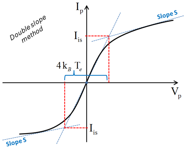
Figure 1. Schematic diagram of the symmetric double probe characteristic to determine T_e in double slope method [43,45].
