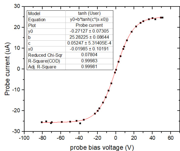
Figure 8. A typical probe characteristic curve at position 2 by 4.5 slm gas flow rate and 26 Watts applied power. Based on the direct fitting method, the hyperbolic tangent curve is fitted on the data and the electron temperature is calculated from the slope at the turning point of the curve (coefficient c ).
