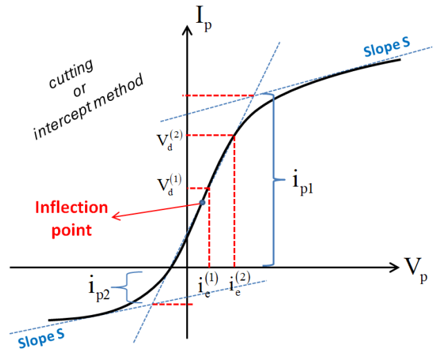
Figure 3. Schematic diagram of the cutting or intercept method to determine T_e from the double probe characteristic curve [44].
