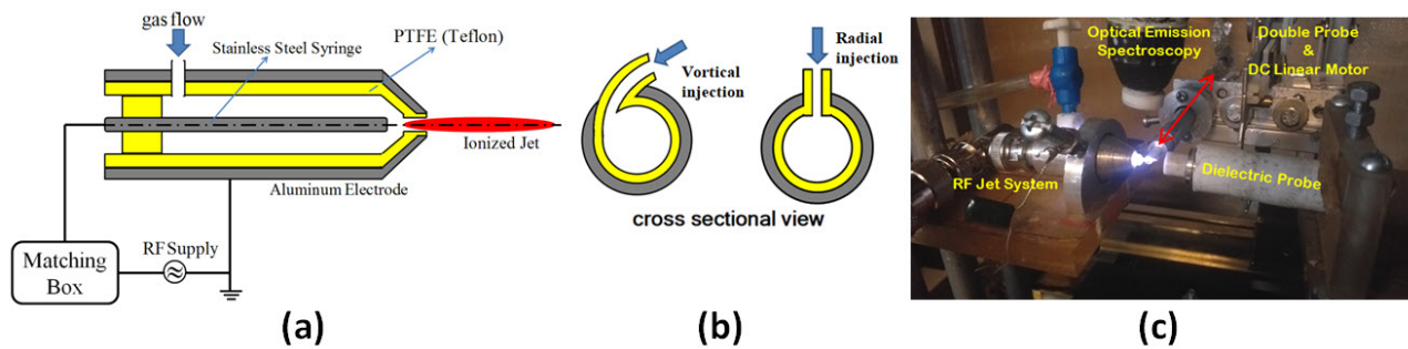
Figure 4. a: Schematic of the designed atmospheric-pressure plasma microjet (APP \mu J), b: gas injection structure, c: an image of the plasma jet and together with the data acquisition system including a spectrometer on the top of the image, dual Langmuir probe on a linear reciprocating system with a DC motor (the front view), and a dielectric probe on the right side of the image (the results of which are not presented in this article).
