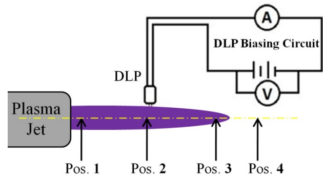
Figure 6. A schematic of the testing layout. The voltage between the two probes from voltmeter can be detected and tuned. Also, the value of the probe current is read from the ammeter or oscilloscope.
