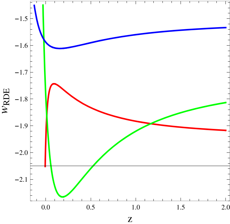
Figure 6 Evolution of w_{RDE} with redshift z . The red, green, and blue lines correspond to c^2 < 0.5, = 0.5, and > 0.5 , respectively.
