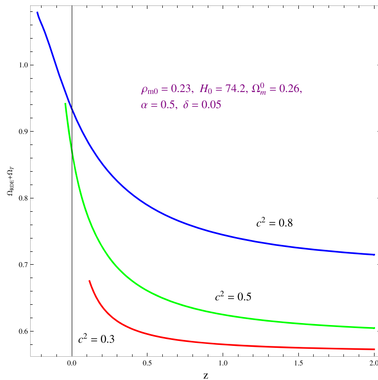
Figure 4 This figure plots the \frac{\Omega_{DE} + \Omega_T}{3\tilde{H}^2} against redshift z . Here, \tilde{H} is the reconstructed Hubble parameter. We have taken \Omega_m^0 = 0.26 and \delta = 0.05 . The red, green, and blue lines correspond to c^2 < 0.5 , = 0.5 , and > 0.5 , respectively.
