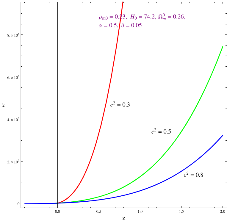
Figure 5 This figure plots the density contribution due to torsion, i.e., \rho_T against redshift z . We have taken \Omega_m^0 = 0.26 and \delta = 0.05 . The red, green, and blue lines correspond to c^2 < 0.5, = 0.5, and > 0.5 , respectively.
