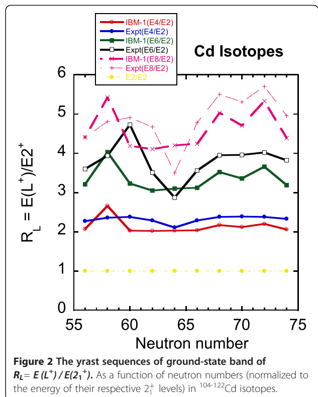
Figure 1 E(4^+)/E(2^+) values as a function of neutron numbers of cadmium isotopes ^{104-122}\text{Cd} . For experimental values, IBM-1, U(5), O(6), and SU(3) limit.
