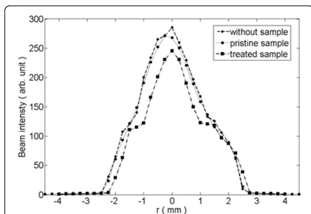
Figure 6 Intensity profiles of the laser beam intensity profiles transmitted through air, pristine, and plasma-treated red BS dye-doped PMMA films.
