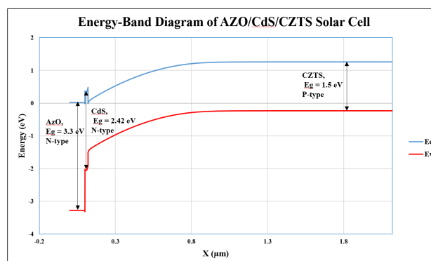
Figure 15. Energy-band diagram of AZO/CdS/CZTS solar cell.
