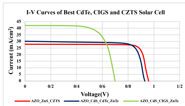
Figure 12. I-V curves of best CdTe, CIGS, and CZTS solar cell.
