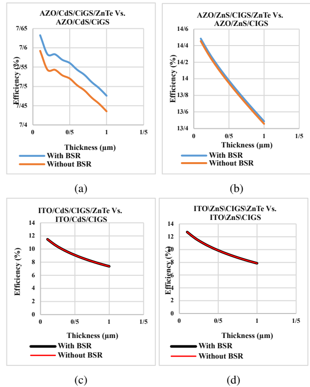
Figure 6. TCO thickness variation with efficiency for CIGS solar cell (a) AZO/CdS/ CIGS /ZnTe (With BSR) Vs. AZO/CdS/ CIGS (Without BSR) (b) AZO/ZnS/ CIGS /ZnTe (With BSR) Vs. AZO/ZnS/ CIGS (Without BSR) (c) ITO/CdS/ CIGS /ZnTe (With BSR) Vs. ITO/CdS/ CIGS (Without BSR) (d) ITO/ZnS/ CIGS /ZnTe (With BSR) Vs. ITO/ZnS/ CIGS (Without BSR).
