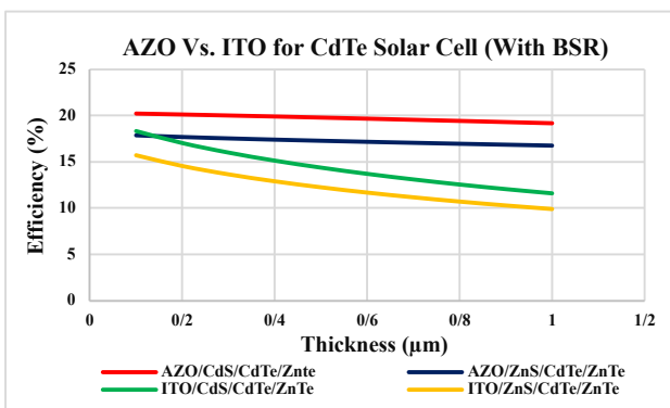
Figure 5. TCO thickness variation for CdTe solar cell.
