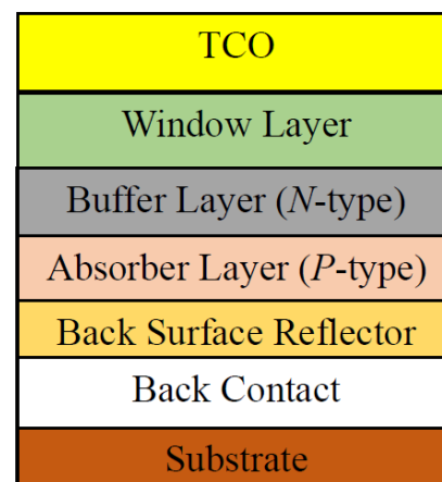
Figure 3. The basic structure of a thin film solar cell where TCO and window layer are separate layers.
