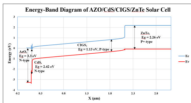
Figure 14. Energy-band diagram of AZO/CdS/CIGS/ZnTe solar cell.
