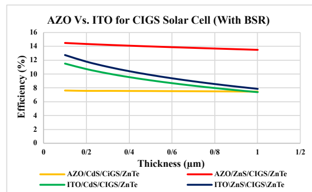
Figure 7. TCO thickness variation for CIGS solar cell.
