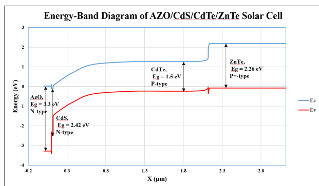
Figure 13. Energy-band diagram of AZO/CdS/CdTe/ZnTe solar cell.
