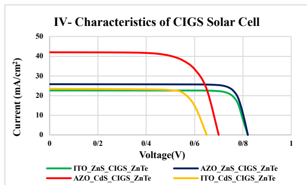
Figure 10. IV- characteristics of CIGS solar cell.
