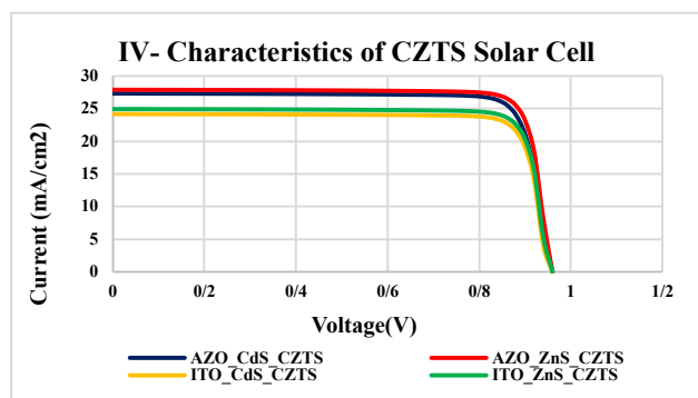
Figure 11. IV- characteristics of CZTS solar cell.
