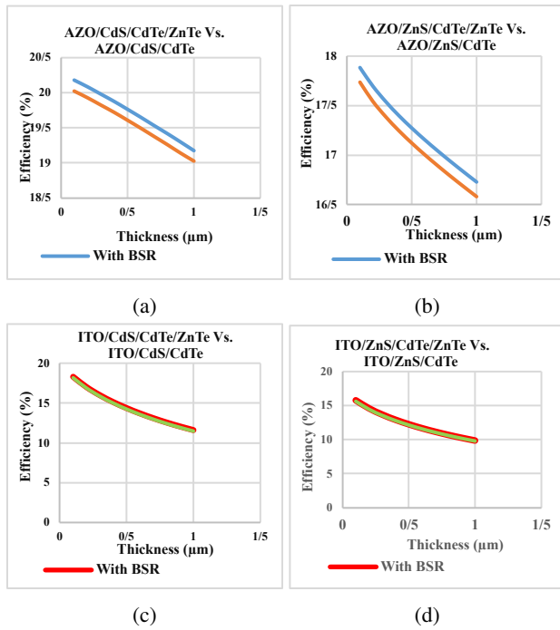
Figure 4. TCO thickness variation with efficiency for CdTe solar cell (a) AZO/CdS/CdTe/ZnTe (With BSR) Vs. AZO/CdS/CdTe (Without BSR) (b) AZO/ZnS/CdTe/ZnTe (With BSR) Vs. AZO/ZnS/CdTe (Without BSR) (c) ITO/CdS/CdTe/ZnTe (With BSR) Vs. ITO/CdS/CdTe (Without BSR) (d) ITO/ZnS/CdTe/ZnTe (With BSR) Vs. ITO/ZnS/CdTe (Without BSR).
