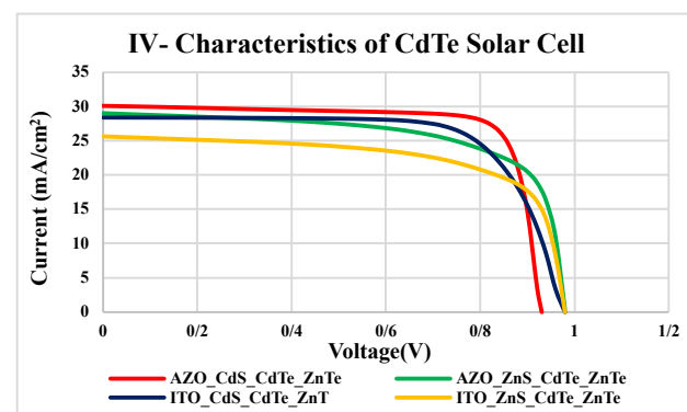
Figure 9. IV- characteristics of CdTe solar cell.
