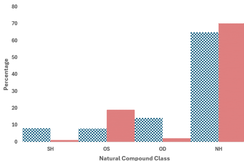
Figure 2. Comparison of the natural compounds groups contributing to the chemical profiles of the essential oils and volatile profiles from the aerial parts of Verbascum sinuatum L. using classical hydrodistillation (CHD) and Headspace-solid phase microextraction (HS-SPME).
