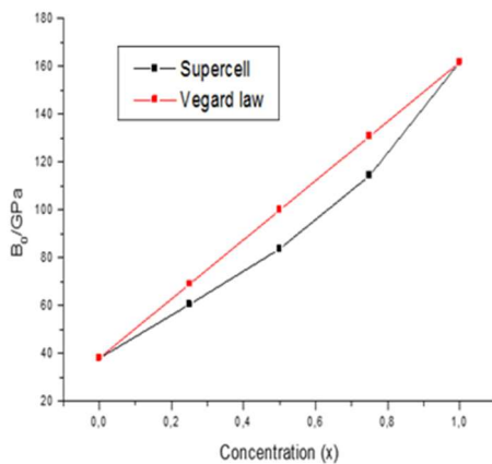
Fig 2. Composition dependence of the calculated bulk modulus of Tl_{1-x}B_xP alloy compared with Vegard's law
