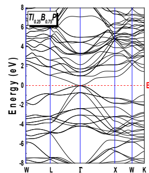
Fig 3. Calculated electronic band structure of Tl_{1-x}B_xP alloy at different compositions ( x = 0.25, 0.5 , and 0.75 ) within the GGA approximation.
