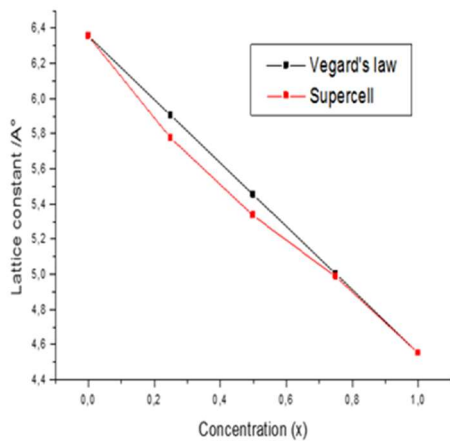
Fig 1. Composition dependence of the calculated lattice constant of Tl_{1-x}B_xP alloy compared with Vegard's law
