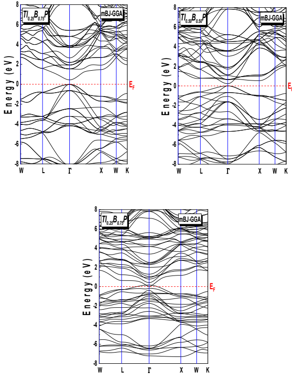
Fig 4. Calculated electronic band structure of Tl_{1-x}B_xP alloy at different compositions ( x = 0.25, 0.5, and 0.75 ) within the Mbj-GGA approximation
