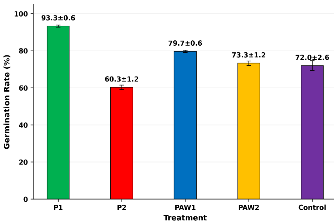
Figure 5. Germination rate (%) of barley seeds on day 7 under direct plasma (P1, P2), plasma-activated water (PAW1, PAW2), and control treatments. Error bars represent the standard error of the mean (SEM)
