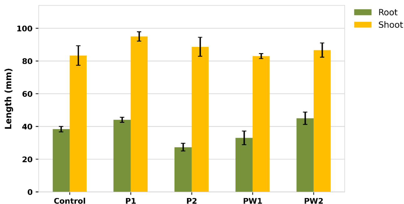
Figure 8. Root and shoot lengths (mm) of barley seedlings on day 14 under different plasma treatments. Error bars represent the standard error of the mean (SEM)
