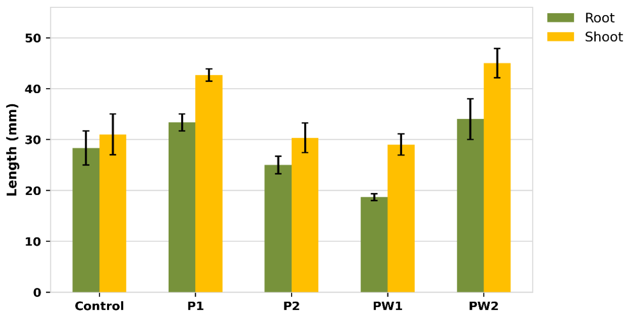
Figure 7. Root and shoot lengths (mm) of barley seedlings on day 9 under different plasma treatments ( P < 0.01 ). Error bars represent the standard error of the mean (SEM)
