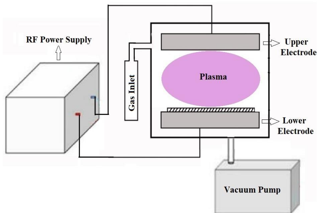
Figure 1. Schematic of the low-pressure glow discharge plasma system used for direct barley seed treatment, operating at 6 \times 10^{-1} Torr with 300 W power and nitrogen gas flow of 2 L/min
