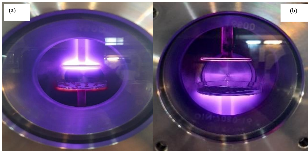
Figure 2. Barley seeds treated with (a) ion-dominated plasma exposure, (b) electron-dominated plasma exposure using low-pressure nitrogen glow discharge ( 6 \times 10^{-1} Torr, 300 W RF, 60 s treatment time)
