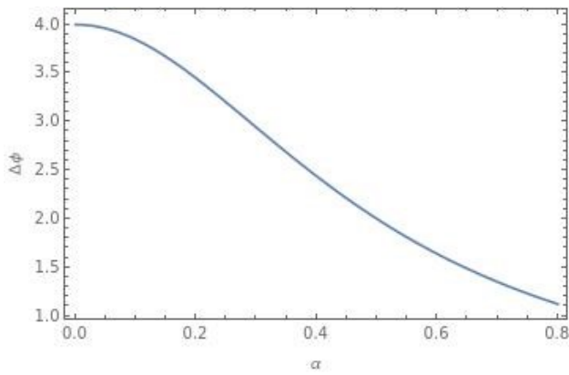
Figure 4. The deflection angle of photon light with cosmic string parameter \alpha for l = 1 = a, \chi = 0.5 .
