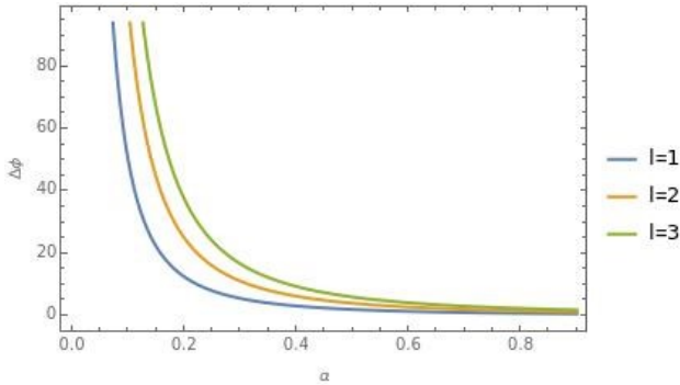
Figure 2. The deflection angle of photon light with cosmic string parameter for fixed value of l . Here \beta = 0.5, a = 1 .
