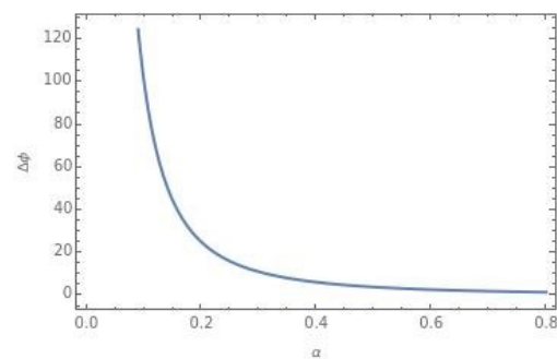
Figure 1. The deflection angle of photon light with cosmic string parameter keeping fixed l . Here \beta = 0.5 , l = 1 = a .
