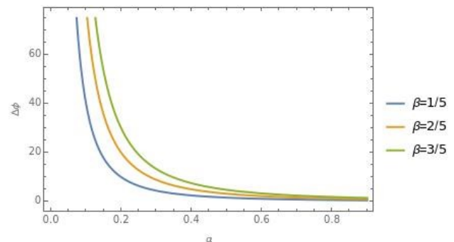
Figure 3. The deflection angle of photon light with cosmic string parameter for different values of screw dislocation parameter \beta . Here l = 1 = a .
