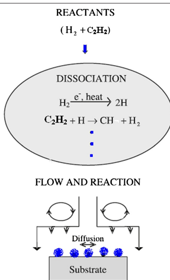
Figure 6 Schematic of the process occurring during diamond CVD by Ni catalyst.
