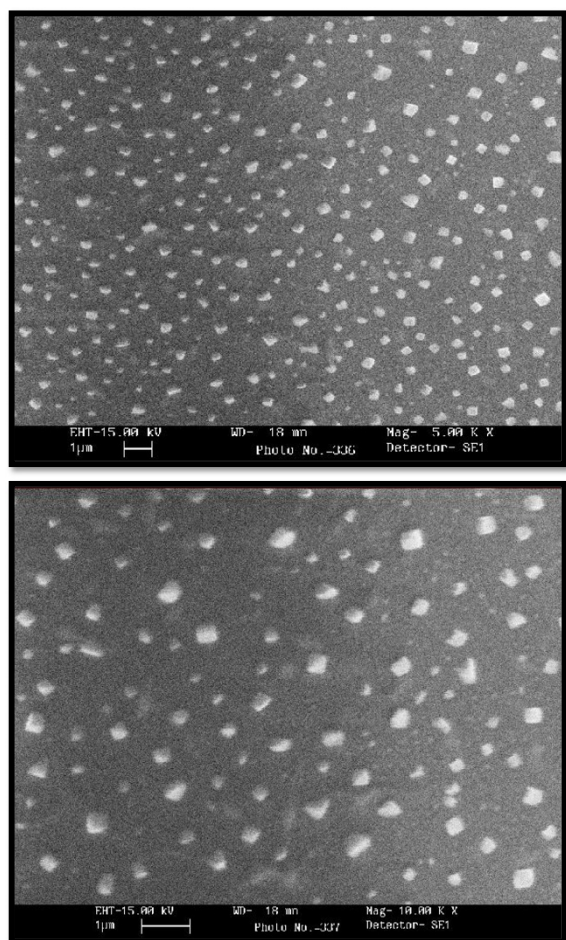
Figure 3 Scanning electron micrograph of nanodiamond synthesized using Ni catalyst on glass substrate.
