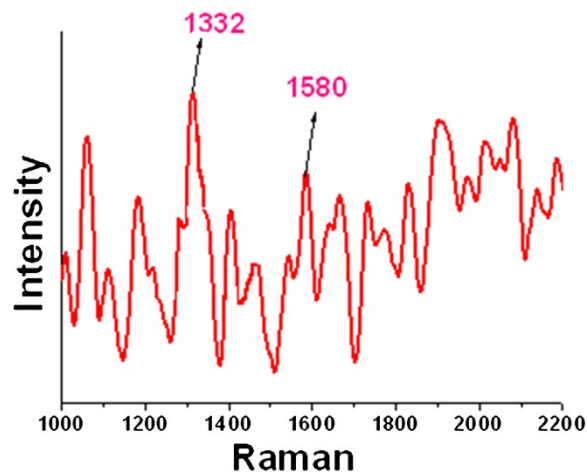
Figure 4 Raman spectra of diamond structure deposited on glass substrate.
