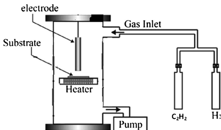
Figure 7 A schematic of plasma-enhanced CVD apparatus.
