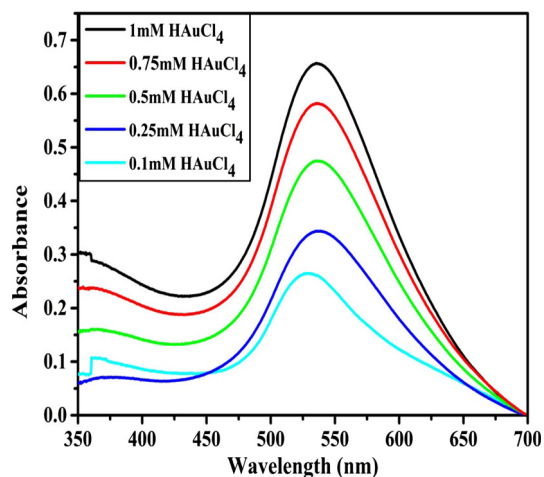
Fig. 2 The UV–Vis absorption spectra of Au nanoparticles synthesized by autoclaving different concentrations of \text{HAuCl}_4 with 0.5 % gum kondagogu solution
