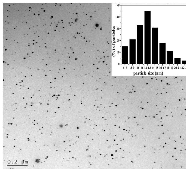
Fig. 5 TEM image of gold nanoparticles synthesized with 1 % (w/v) gum kondagogu and 1 mM \text{HAuCl}_4 , autoclaved for 15 min at 15 psi and histogram showing the particle size distribution
