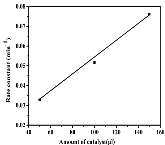
Fig. 9 Plot of rate constant ( k ) versus amount of AuNPs for the reduction reaction of 4-NP by \text{NaBH}_4 in the presence of AuNPs as catalyst. Conditions: [4-NP] = 0.2 mM; [\text{NaBH}_4] = 15 mM; different amounts of gold nanoparticles obtained from 1 mM of chloroauric acid and 0.5 % of gum kondagogu
