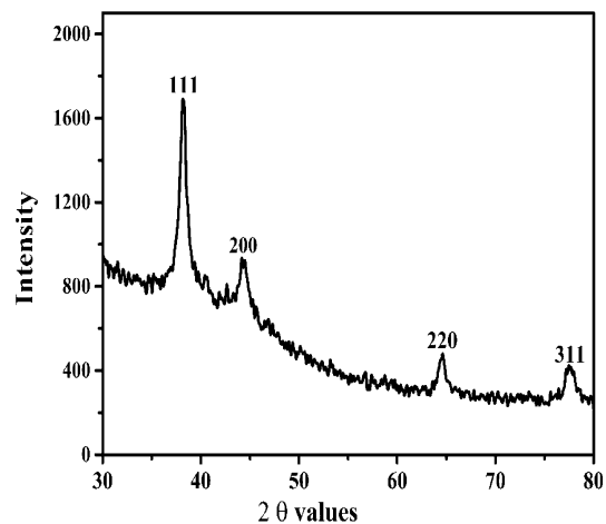
Fig. 4 XRD pattern of gold nanoparticles stabilized in gum kondagogu. Conditions: 0.5 % (w/v) of gum solution, 1 mM \text{HAuCl}_4 and autoclaved for 15 min at 15 psi
