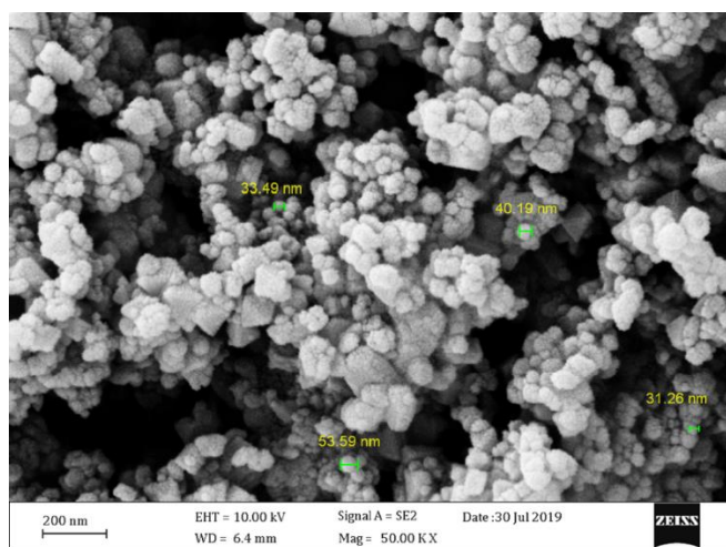
Fig. 2. SEM image of synthesized nano-catalyst
