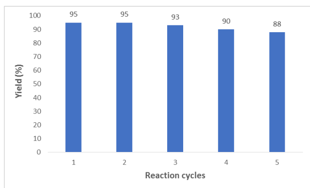
Fig. 6. The reusability of the synthesized nano-catalyst
