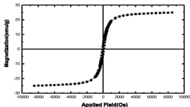
Fig. 5. The VSM curve of synthesized nano-catalyst
