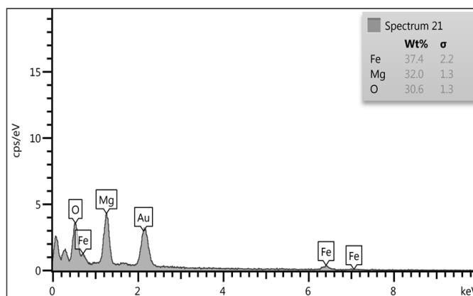
Fig. 4. The EDS analysis of synthesized nano-catalyst
