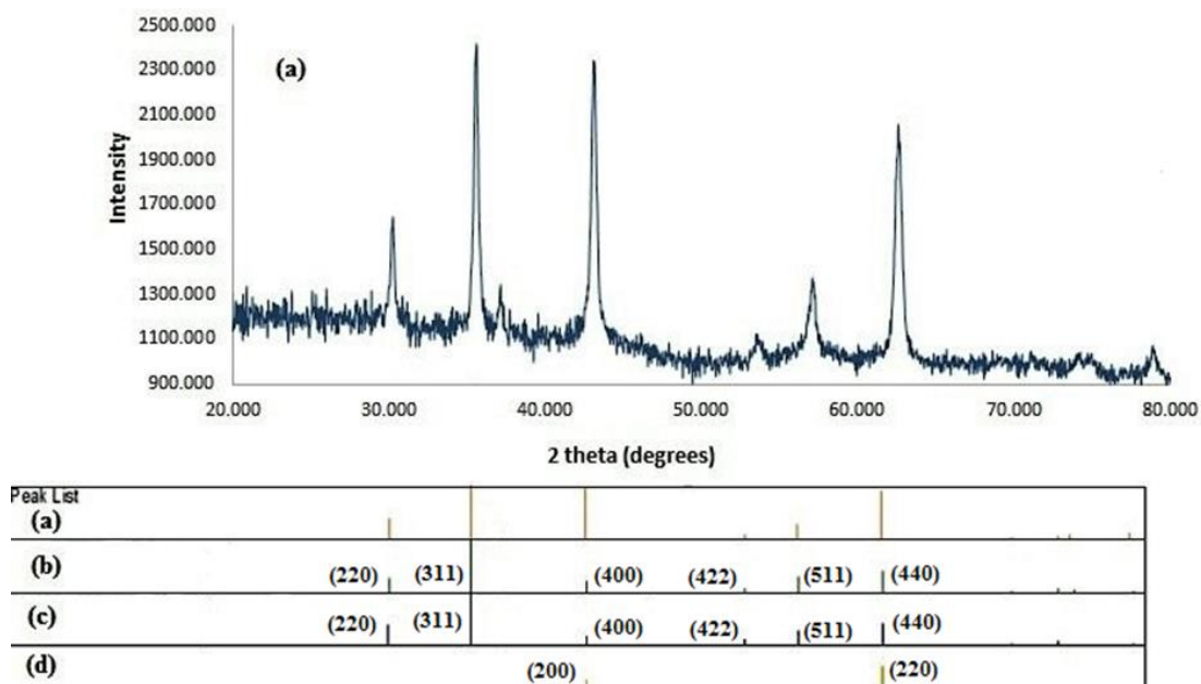
Fig. 1. The powder X-ray diffraction patterns of: a) synthesized Mg-Fe bi-metal catalyst, b) standard MgFe_2O_4 , c) standard Fe_3O_4 d) standard MgO
