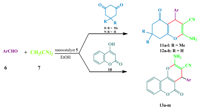
Scheme 2. Synthesis of chromene derivatives using [\gamma\text{-Fe}_2\text{O}_3\text{@HAp-Si}(\text{CH}_2)_3\text{BF}_4\text{@DMIM}] ( 5 )
