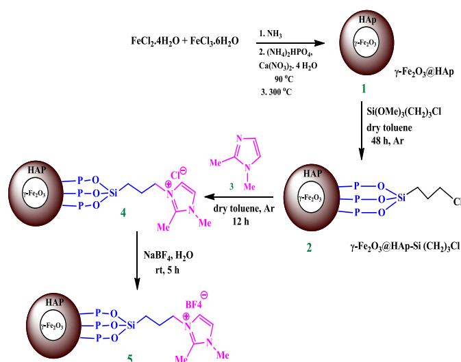
Scheme 1. Synthesis of [\gamma\text{-Fe}_2\text{O}_3\text{@HAp-Si(CH}_2\text{)}_3\text{BF}_4\text{@DMIM}] (5).
