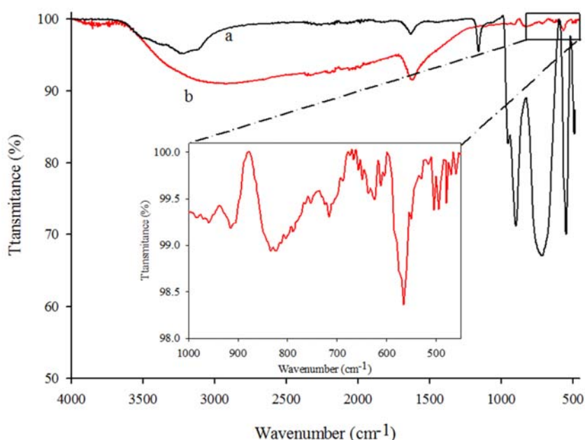
Fig. 1. FT-IR spectra of (a) pure \text{InVO}_4 and (b) \text{InVO}_4\text{-TiO}_2 . Inset shows the enlarged view of the peaks of \text{InVO}_4\text{-TiO}_2 in 1000\text{-}450\text{ cm}^{-1} .
