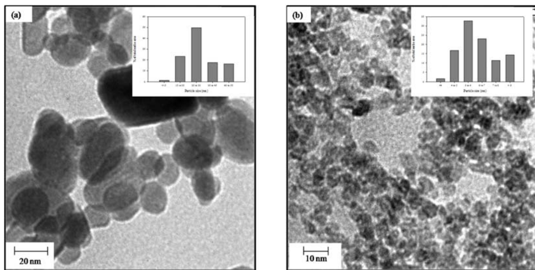
Fig. 4. TEM images and particle size histograms of (a) pure InVO 4 and (b) InVO 4 -TiO 2 nanocomposite.
