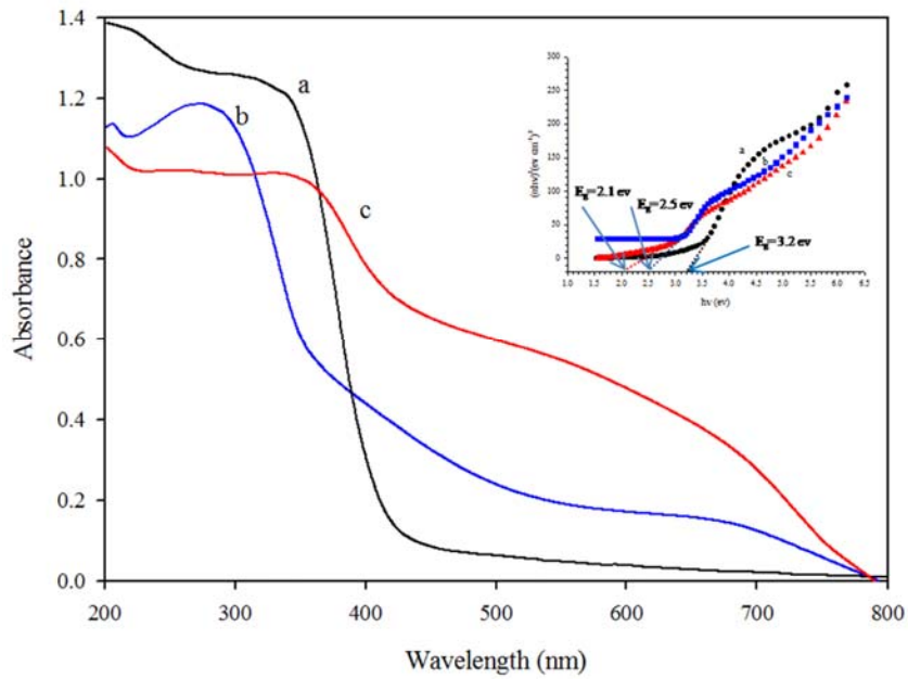
Fig. 2. UV-vis diffusion reflectance spectra of (a) pure TiO 2 , (b) pure InVO 4 [33] and (c) InVO 4 -TiO 2 [33]. Inset shows the Tauc plot for band gap energy determination of (a) pure TiO 2 , (b) pure InVO 4 and (c) InVO 4 -TiO 2 .
