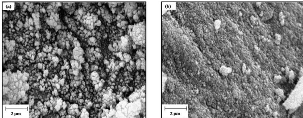
Fig. 3. SEM micrographs of (a) pure InVO 4 and (b) InVO 4 -TiO 2 nanocomposite [33].
