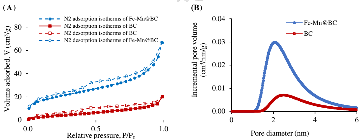
Fig 1. (A) Nitrogen adsorption–desorption isotherms at 77 K of BC and Fe-Mn@BC; (B) Pore size distribution of BC and Fe-Mn@BC
