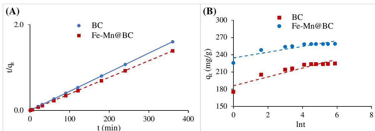
Figure SM1. Linearized pseudo second-order (A) and Elovich (B) kinetics for adsorption of Pb 2+ onto BC and Fe-Mn@BC
