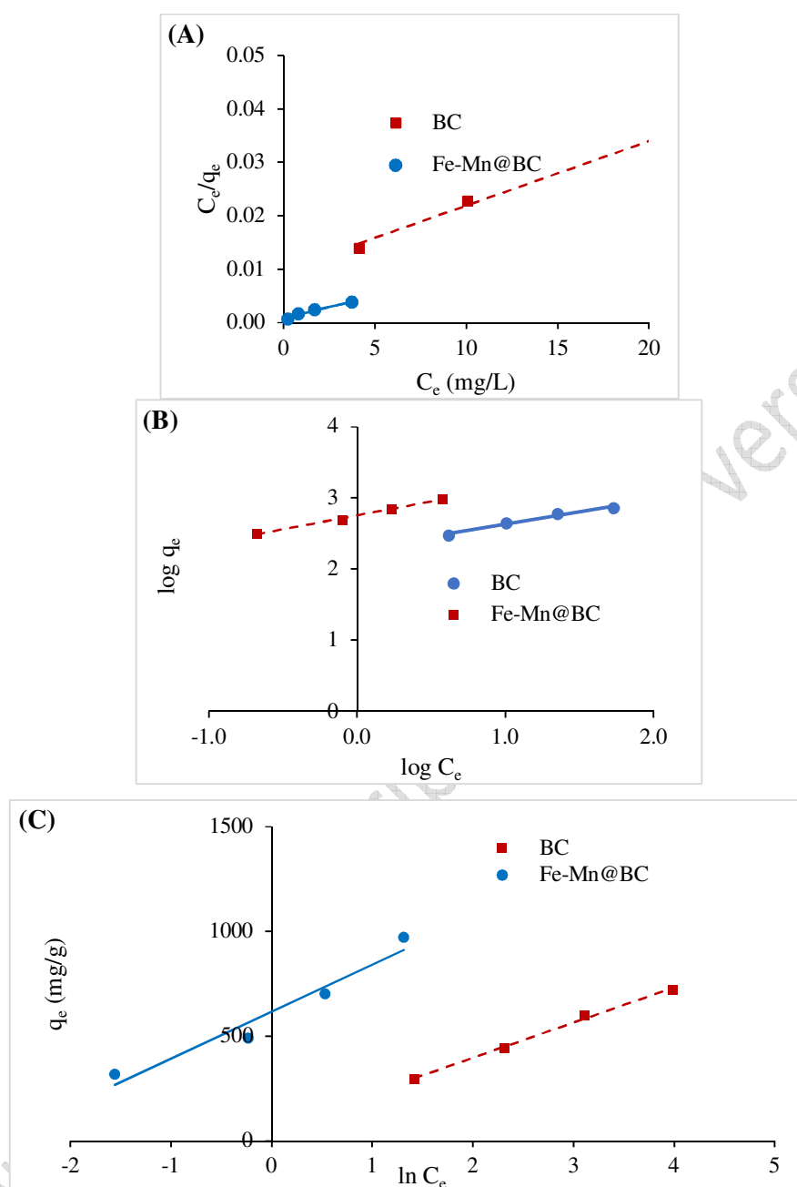
Figure SM3. Linearized Langmuir (A), Freundlich (B), and Temkin (C) isotherms for adsorption of Pb^{2+} onto BC and Fe-Mn@BC
