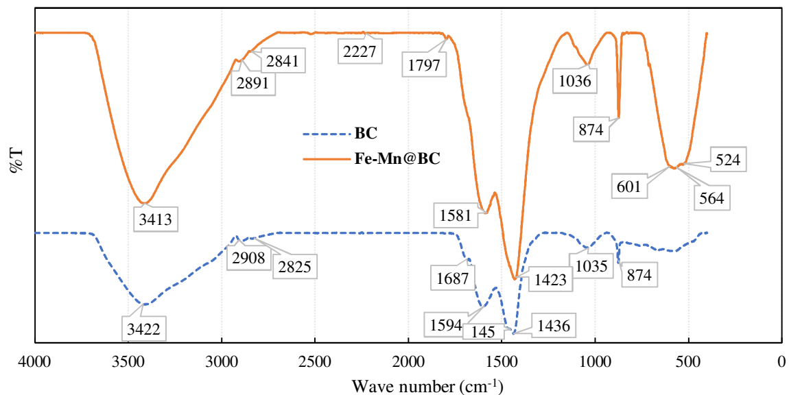
Fig 2. The FT-IR spectra of BC and Fe-Mn@BC
