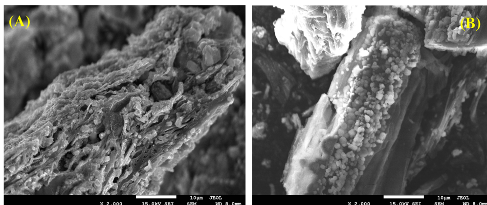
Fig 3. The SEM images of BC (A) and Fe-Mn@BC (B)
