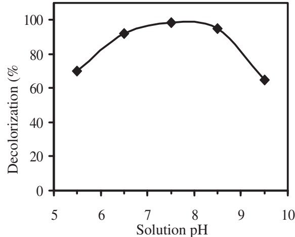
Figure 6 Effect of initial solution pH on decolorization of BGY. BGY = 20 mg/L, catalyst loading = 6 g/L, illumination time = 2 h.
