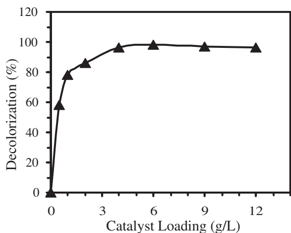
Figure 5 Effect of catalyst loading on decolorization of BGY. BGY = 20 mg/L, pH approximately 7; illumination time = 2 h.
