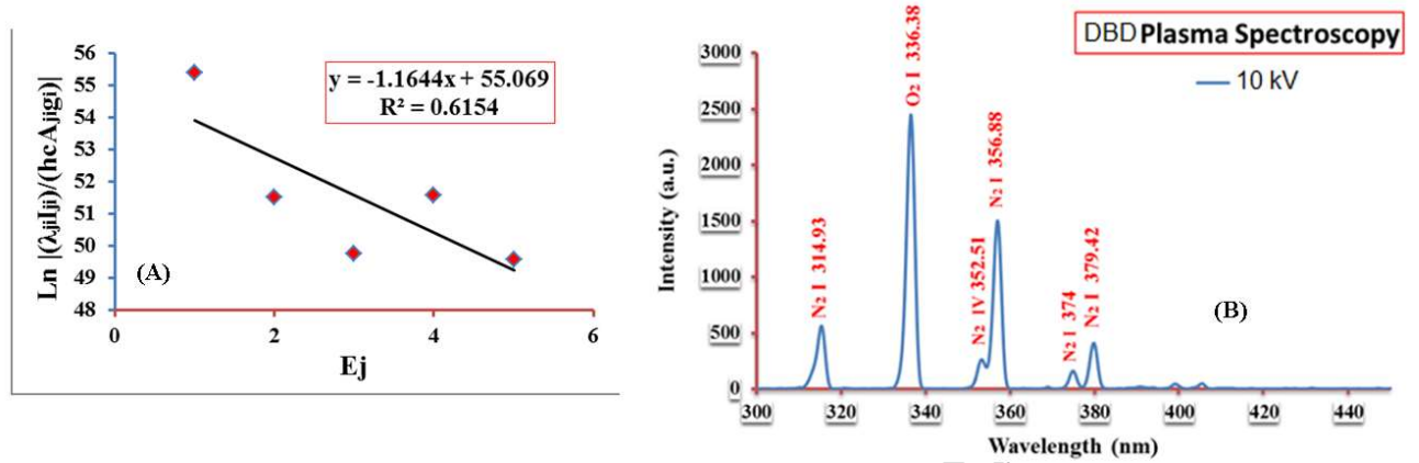
Fig. 1: A) Boltzmann plots for 10 kV applied voltage of DBD plasma system, B) DBD plasma system Spectrum at AC applied voltage of 10 kV
