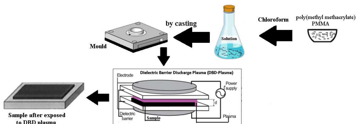
Fig. 2: The PMMA/TiO 2 nanocomposite films when focused by DBD plasma system
