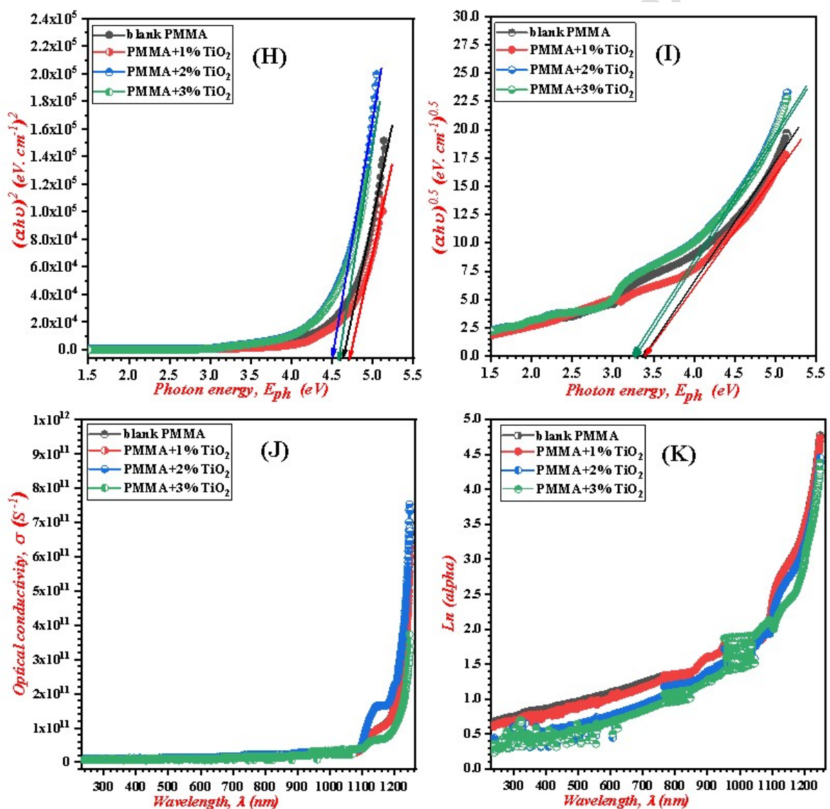
Fig. 5: H) Direct energy gap transition, I) Indirect energy gap transition, J) Optical conductivity, and K) Urbach energy
