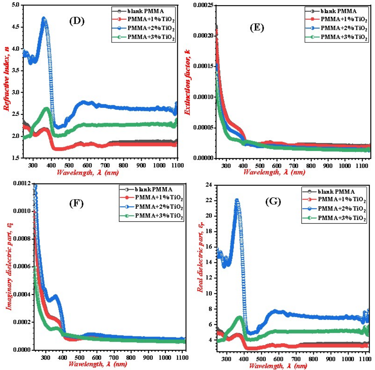
Fig. 4: D) Refractive index, E) Extinction factor, F) Imaginary dielectric part G) Real dielectric part
