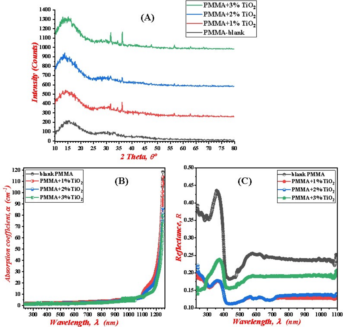
Fig. 3: A) XRD diffraction of PMMA/TiO 2 nanocomposite pattern, B) absorption coefficient, C) reflectance
