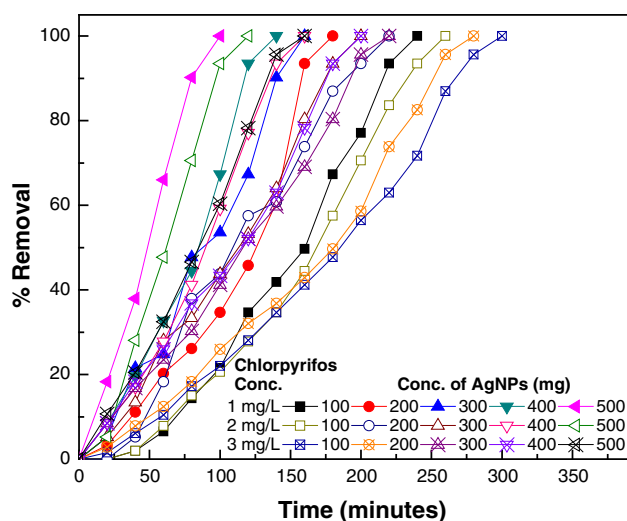
Fig. 3 Mineralization of chlorpyrifos at different AgNP concentration
