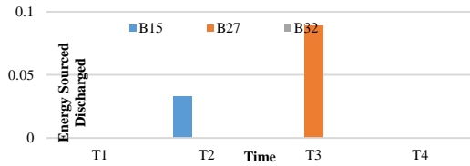
Fig. 11. Discharging schedule of the storage in BC and islanded mode.
