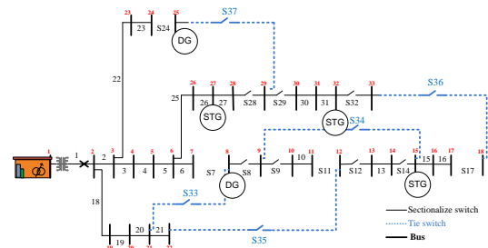
Fig. 5. New network structure after reconfiguration and placement of storage and distributed generation sources in the connected mode.
