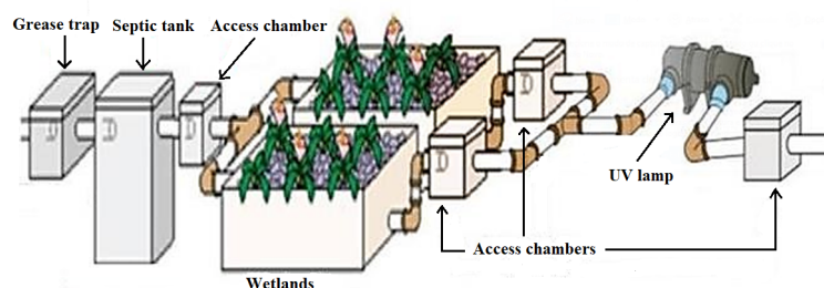
Figure 2. Diagram of the WWTP on the Campus of Araras, UFSCar. Source: Garay et al. (2021).
