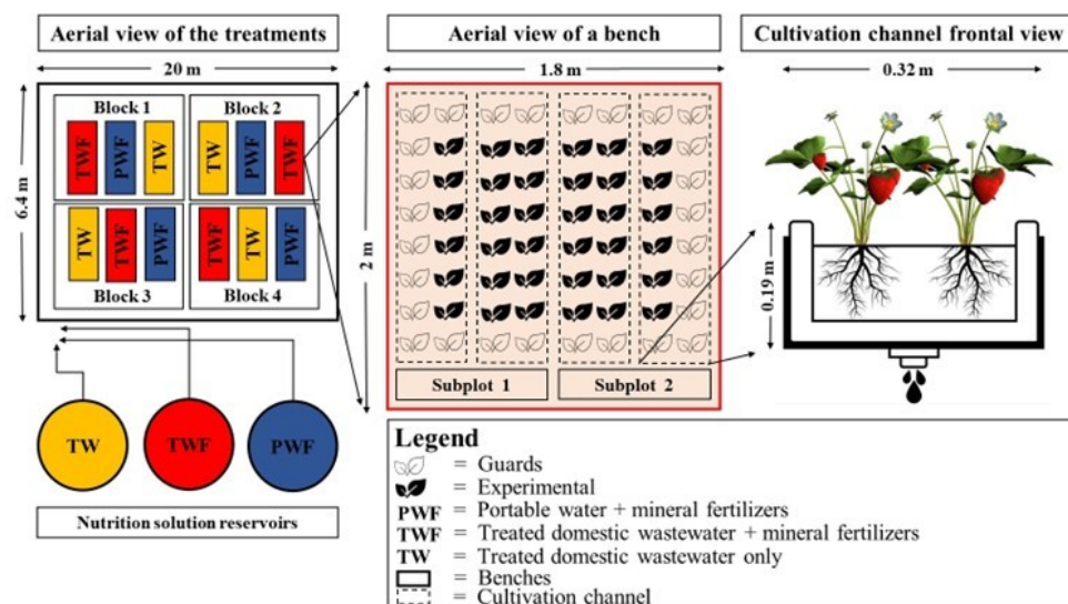
Figure 1. Diagram of the strawberry substrate cultivation system.
