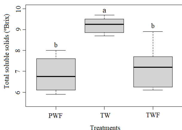
Figure 6. Boxplot and Tukey test for averages of total soluble solids (°BRIX).
