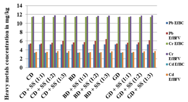
Figure 2. Concentration of heavy metals (mg/kg) of earthworm Eisenia fetida body in different of combination animal dung with sewage sludge after vermicomposting.
