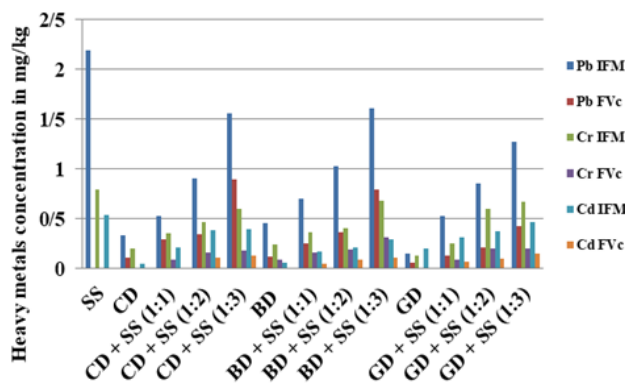
Figure 1. Concentration of heavy metals (mg/kg) in combination of different animal dung with sewage sludge in initial feed mixture and vermicompost.
