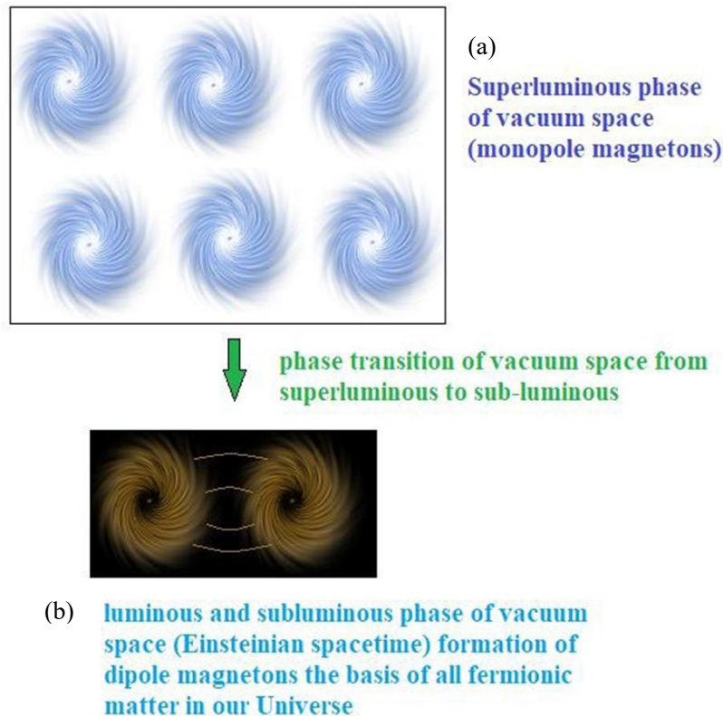
Figure 1. (a) Schematic showing superluminous phase of vacuum space, monopole magnetons [53-56] essentially “empty space”, manifesting subsequent phase transitions. (b) Schematic sketching of phase transitioned luminous and subluminal phase of vacuum space, Einsteinian spacetime formation of dipole magnetons [53-56].
