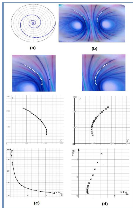
Figure 2. (a) A logarithmic spiral. (b) QFM vortex dipole field magnetism. (c) left arm of spiral segment of the QFM. (d) Right arm spiral segment, these measurements comparatively show real-time observations originally per Figure 6 [53], measurements with the Ferrolens [53].
