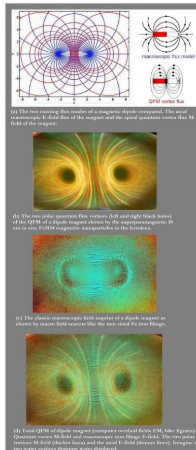
Figure 3. Physical mechanism for explaining classical macroscopic E-field of macro vacuum quantum field dipole magnetism with vortex casualty effect originally Figure 6 [53].
