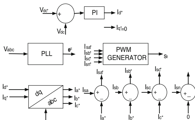
Fig. 2 Inverter controller for current compensation
