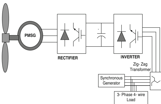
Fig. 3 Schematic with zig-zag compensation
