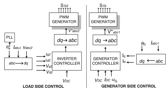
Fig. 4 Converter control
