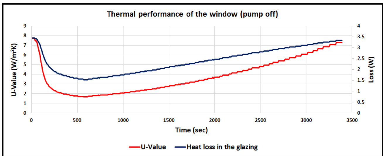
Fig. 10 Glazing U-value and heat loss in scenario 1
