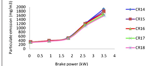
Figure 16 Variation of particulate emission with brake power.
