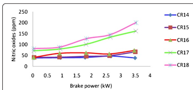
Figure 15 Variation of NO x emission with brake power.
