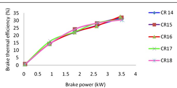
Figure 3 Variation of brake thermal efficiency with brake power.
