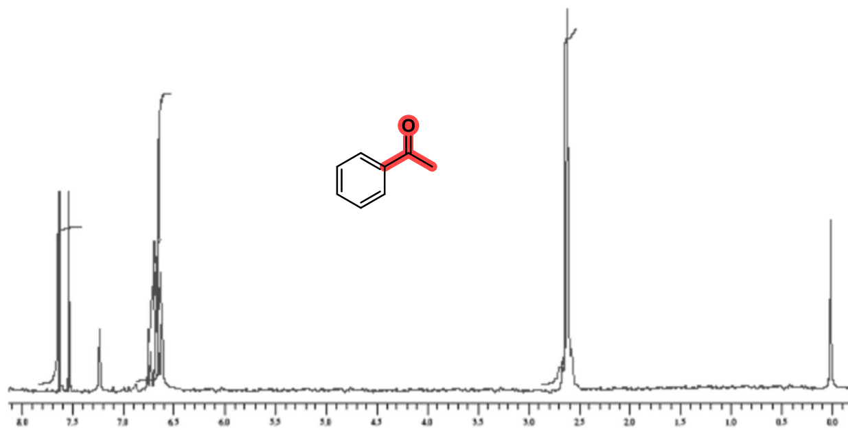
Figure S4. 1 H NMR spectrum of compound 2i
