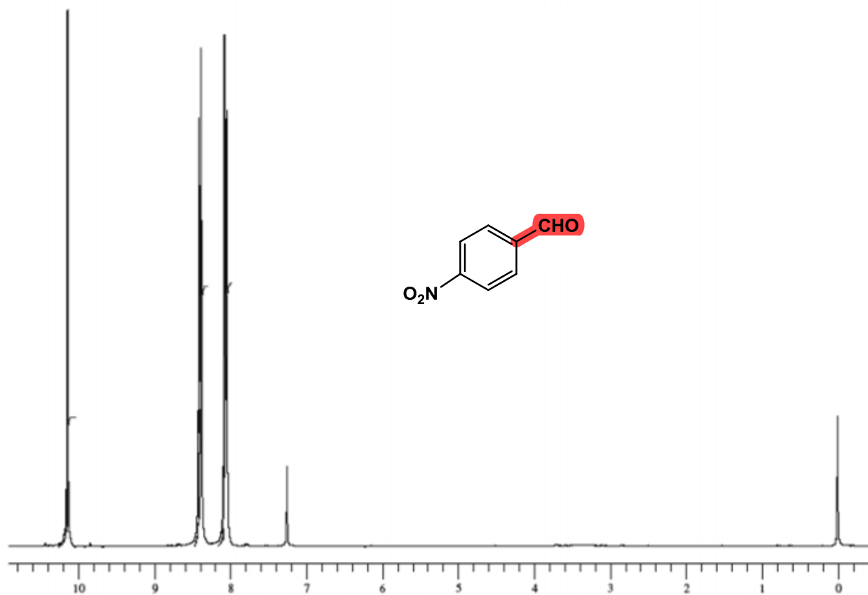
Figure S3. 1 H NMR spectrum of compound 2g
