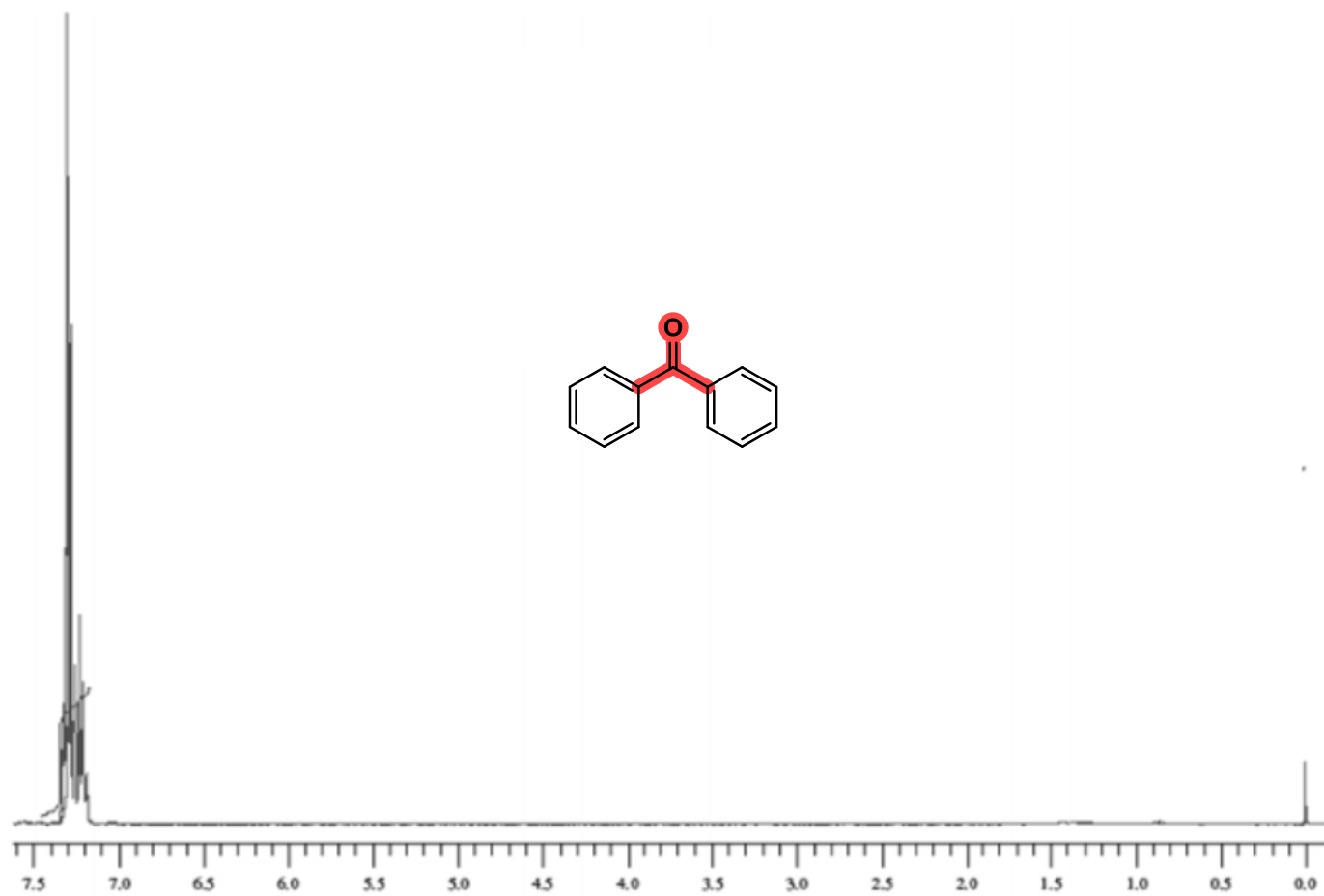
Figure S5. 1 H NMR spectrum of compound 2k
