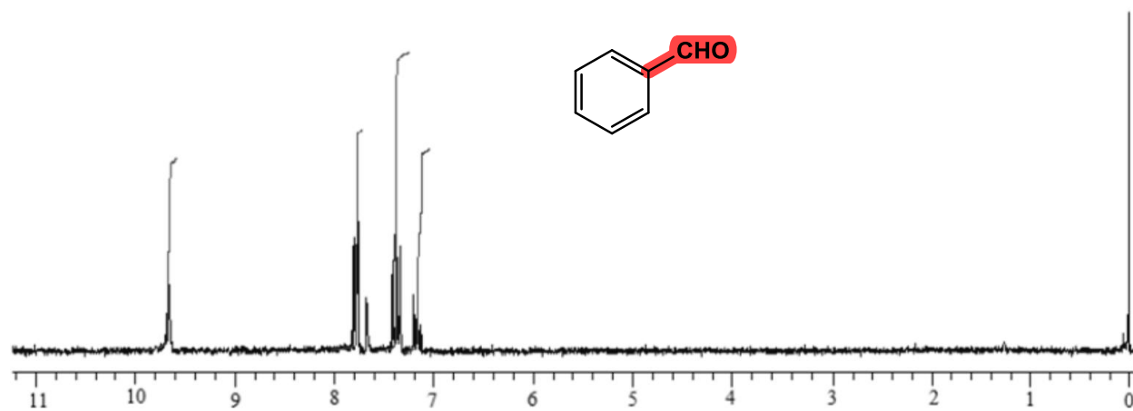
Figure S1. 1 H NMR spectrum of compound 2a
