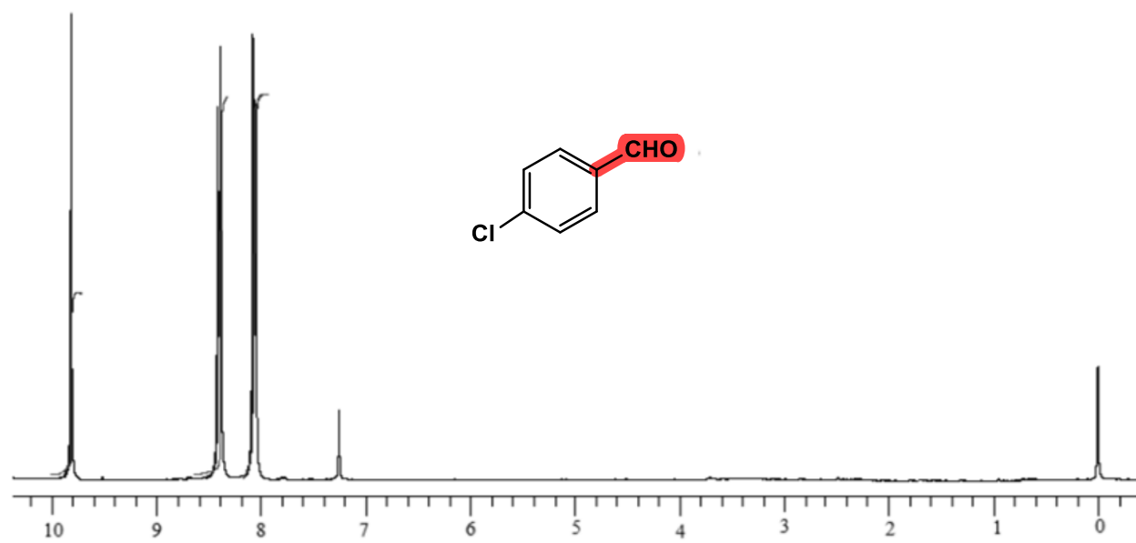
Figure S2. 1 H NMR spectrum of compound 2b
