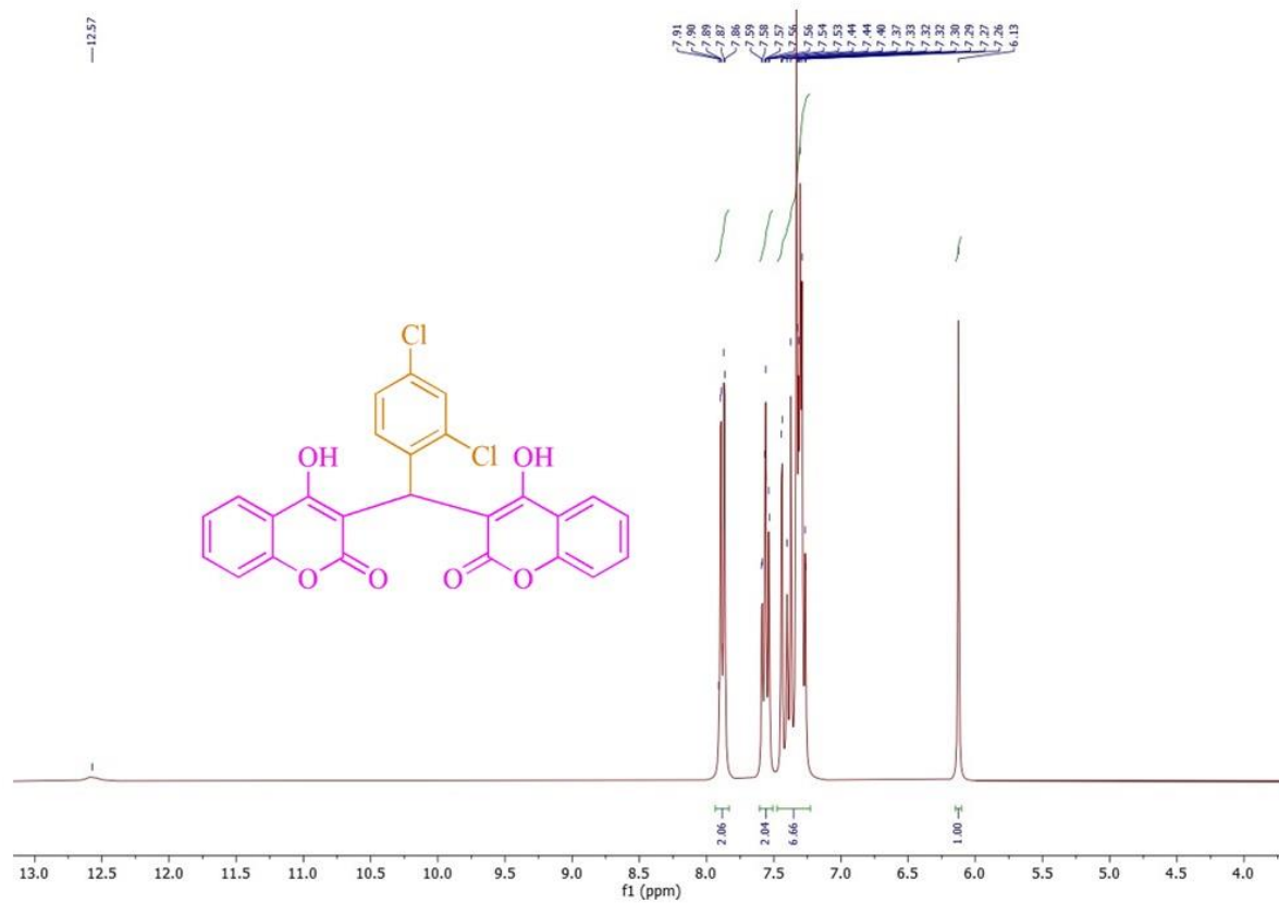
Figure 2s. ^1\text{H} NMR spectrum of 3k in DMSO- d_6 solvent
