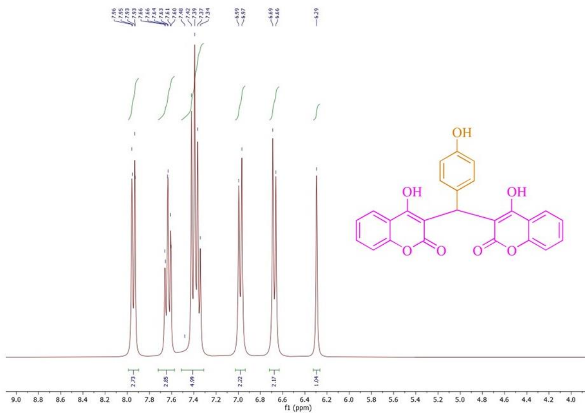
Figure 1s. ^1\text{H} NMR spectrum of 3c in \text{DMSO-d}_6 solvent
