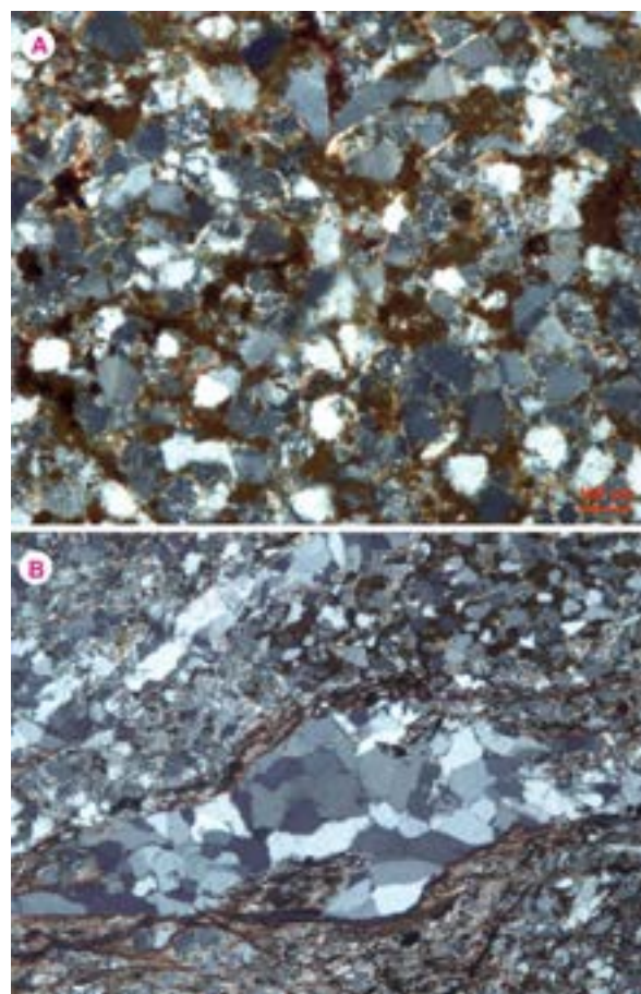
Figure 6. Petrological features of Lower–Middle Jurassic sandstones in thin sections (P.P.L.): A) general view (100 µm scale bar is in the lower right angle), B) secondary quartz grains filling joint-related cavities (200 µm scale bar is in the lower right angle).
