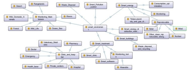
Figure 5. How to inherit the components of the smart environment
