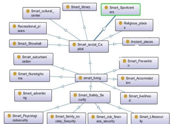
Figure 9. Classes and their inheritance in smart life
