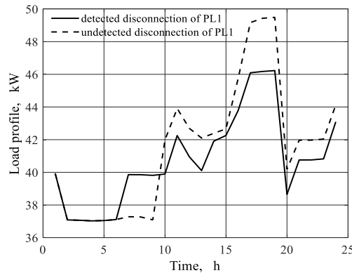
Fig. 5. Simulation results for parking lot 1 in detected and undetected disconnection.
