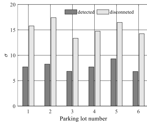
Fig. 10. Variance values of different parking lots in detected disconnection and undetected disconnection.
