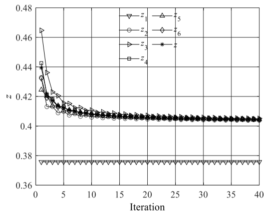
Fig. 8. Simulation results for parking lot 1 in detected disconnection at 8 a.m. and convergence of other parking lots.
