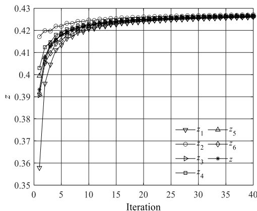
Fig. 9. Simulation results for parking lot 1 in connected condition at 12 and convergence of all parking lots.
