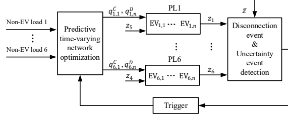
Fig. 2. Schematic of event-based predictive optimization.
