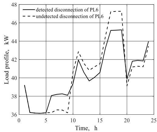
Fig. 7. Simulation results for parking lot 6 in detected and undetected disconnection.
