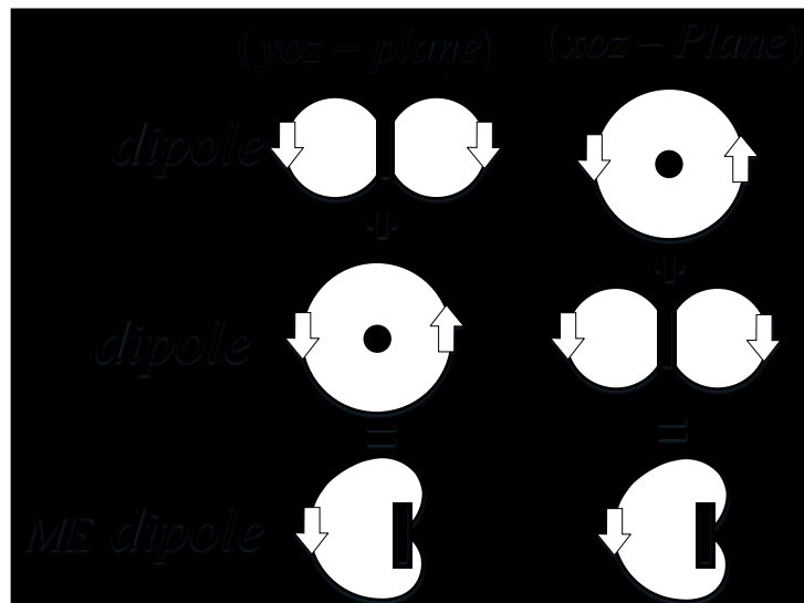
Fig. 2. Radiation mechanism of magneto-electric dipole antenna.
