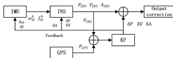
Fig. 2. Structure of the loosely coupled inertial navigation system[21].
