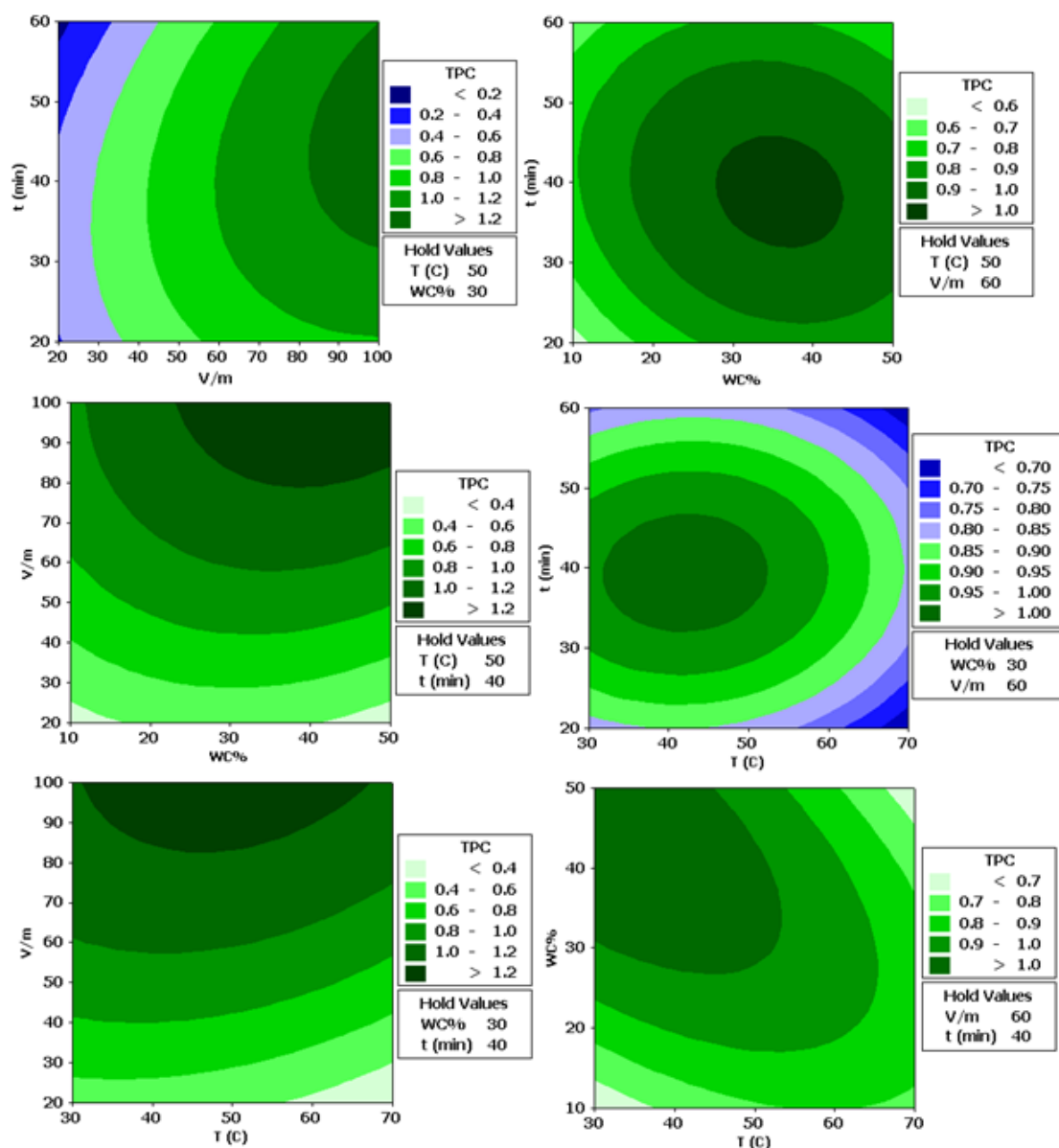
Figure 7. Contour plots of TPC vs. extraction variables.
