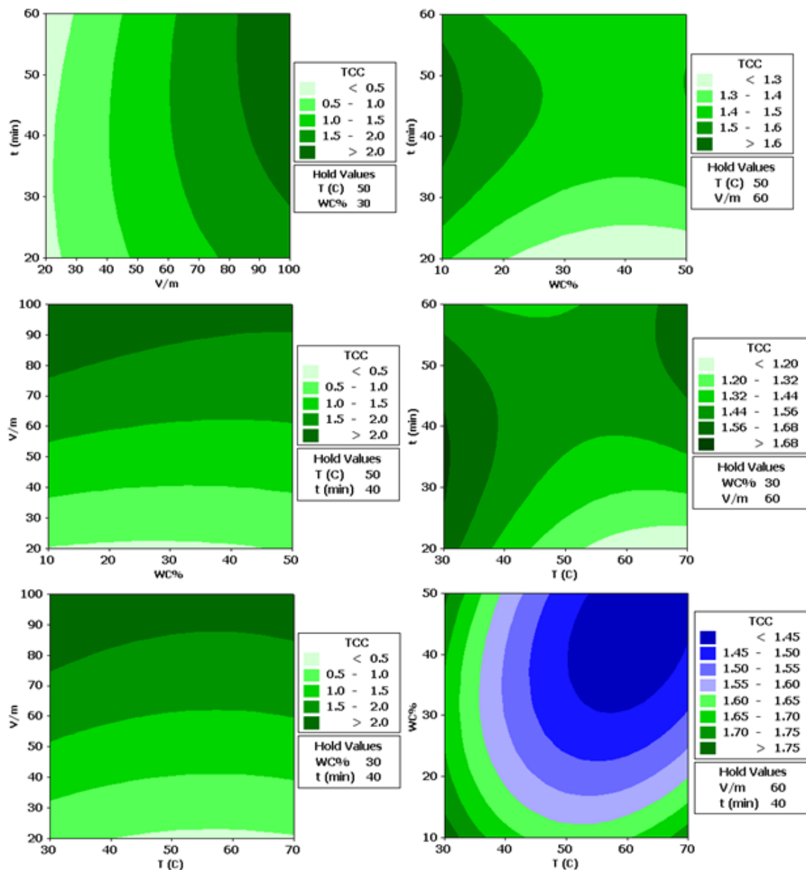
Figure 4. Contour plots of TCC vs. extraction variables.
