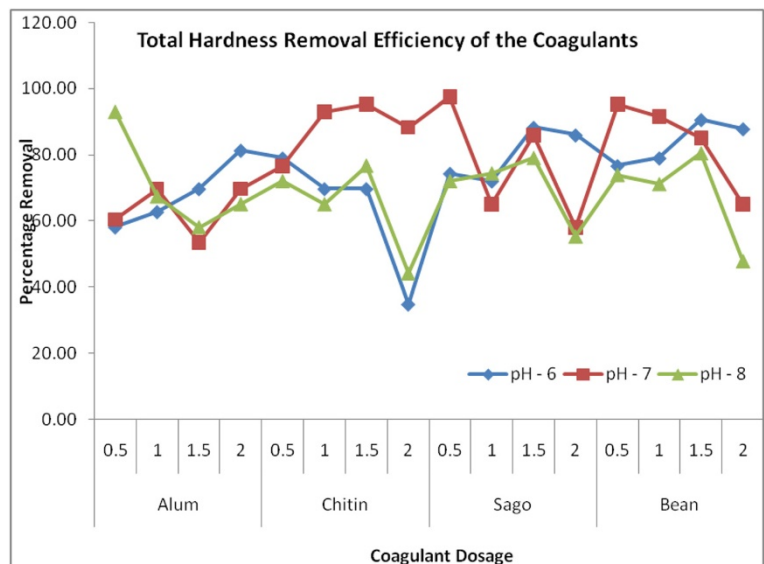
Figure 7 Total hardness removal efficiency of individual coagulants.
